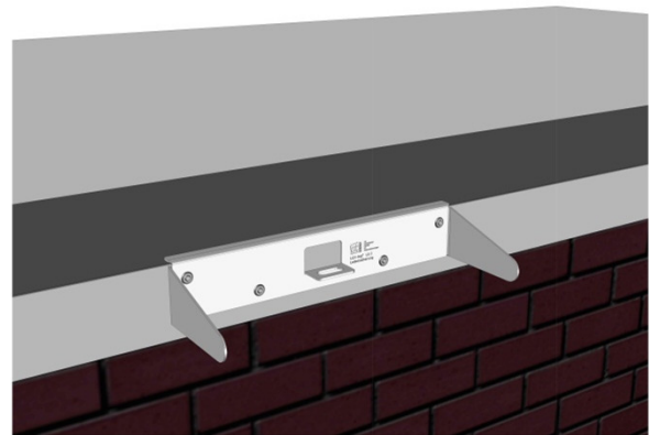
Illust. 1: LUX-top® LS I mounted on the parapet sheet
